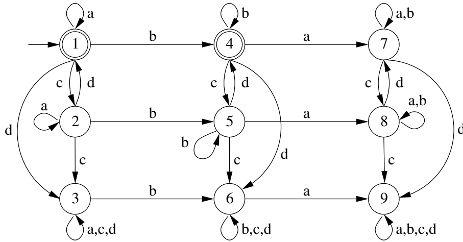
FIGURE II.22. AFD "shuffle".
