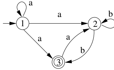
FIGURE II.24. Un AFND.
