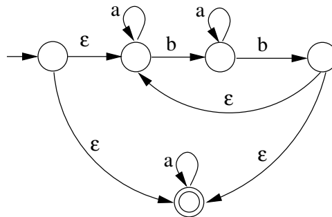
FIGURE III.11. AFND acceptant (\{a\}^*\{b\}\{a\}^*\{b\})^*\{a\}^* .
